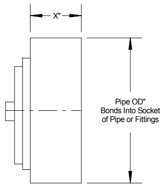
Cleanout Bushing
