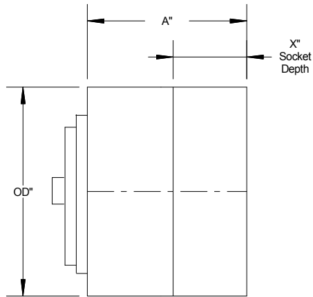
Cleanout Endcap
