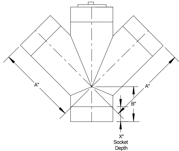
45 deg Double Lateral with Cleanout Position 2
