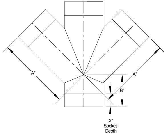
45 deg Double Lateral with Cleanout Position 2
